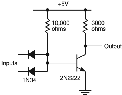
FIGURE 160. NAND gate built with transistors and diodes
