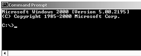
FIGURE 62. Command prompt
