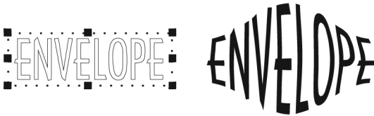
FIGURE 94. Envelope manipulation
