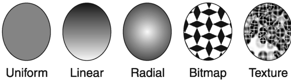
FIGURE 102. Fills
