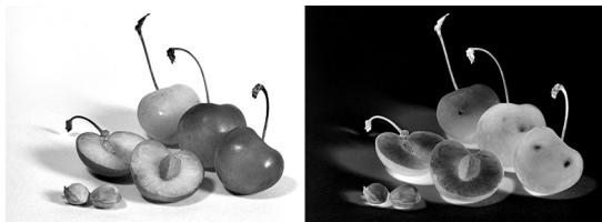
FIGURE 176. Negative image
